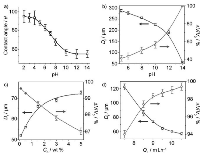
Figure 3. a) Variation in contact angle of an aqueous solution of NaOH in air on the PS-co-PAA film, measured at different pH values. b–d) Effect of experimental variables on the final diameter D_f of armored bubbles (□) and on the fractional change in volume of the \text{CO}_2 plugs (○). b) Effect of initial pH value of the continuous phase at P_{\text{CO}_2} = 4.5 \text{ psi} , C_p = 1.5 \text{ wt}\% , Q_L = 9.5 \text{ mL h}^{-1} . c) Effect of C_p at P_{\text{CO}_2} = 5 \text{ psi} , pH 14, Q_L = 10.0 \text{ mL h}^{-1} . d) Effect of the flow rate Q_L of the continuous phase, P_{\text{CO}_2} = 5 \text{ psi} , pH 14, C_p = 1.5 \text{ wt}\% .
